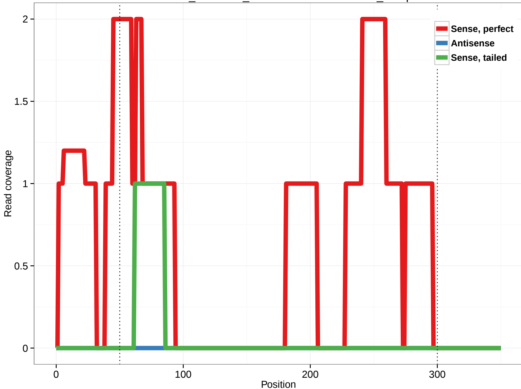
ornAna1_ensGene_ENSOANT00000011788_20.3p
