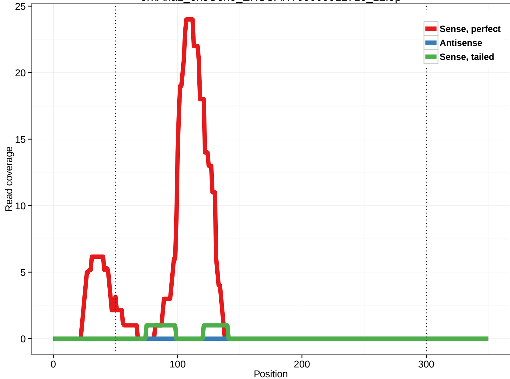
ornAna1_ensGene_ENSOANT00000011716_12.5p
