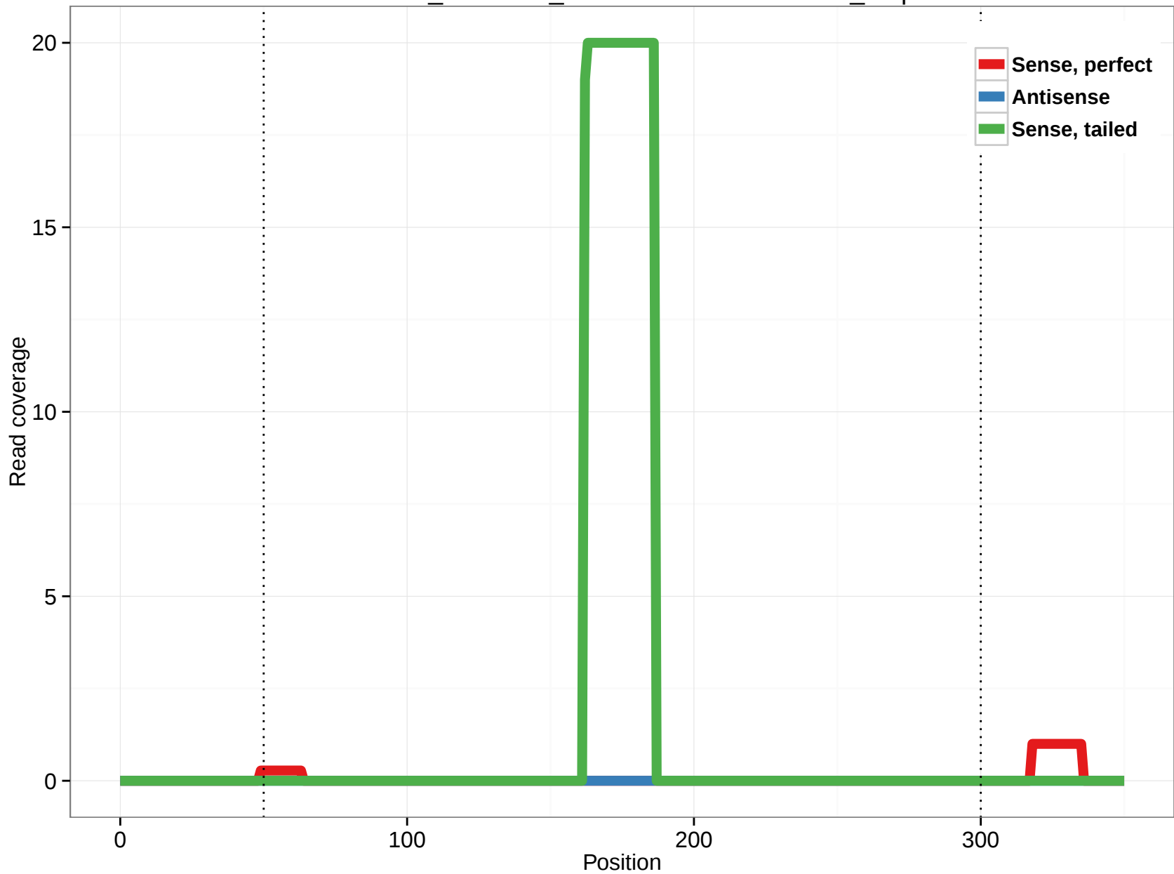
ornAna1_ensGene_ENSOANT00000011712_5.3p
