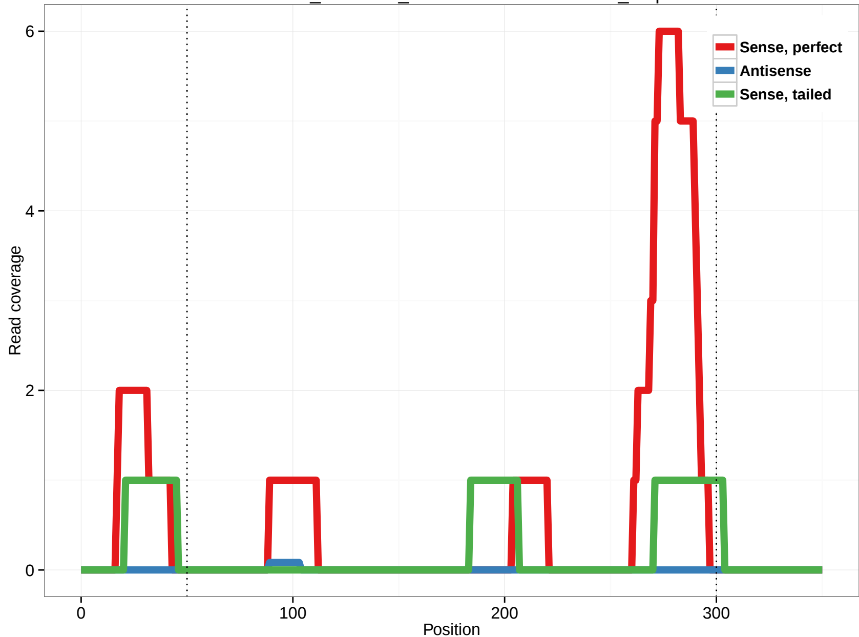
ornAna1_ensGene_ENSOANT00000011659_5.5p
