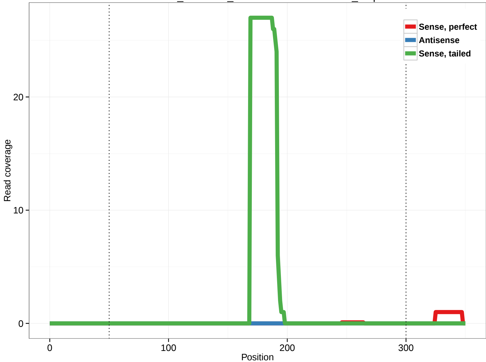
ornAna1_ensGene_ENSOANT00000011625_1.3p
