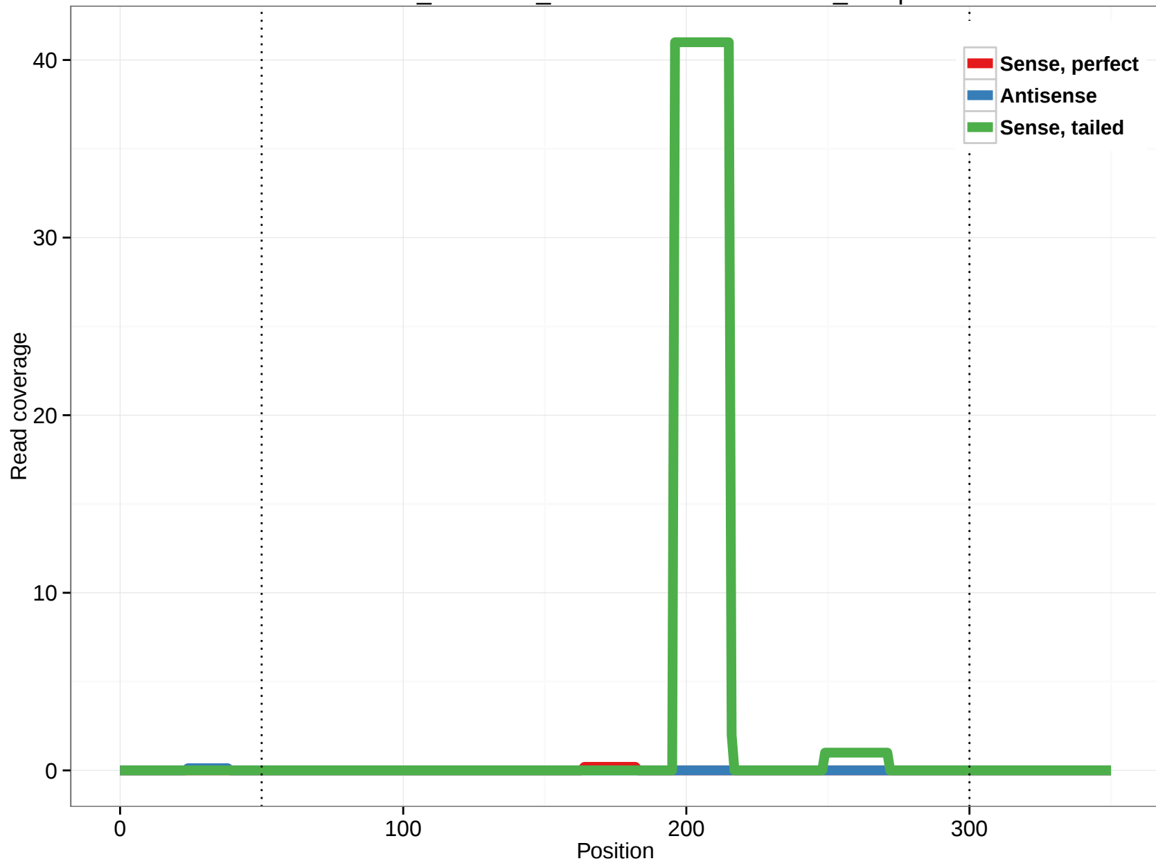
ornAna1_ensGene_ENSOANT00000011546_11.5p
