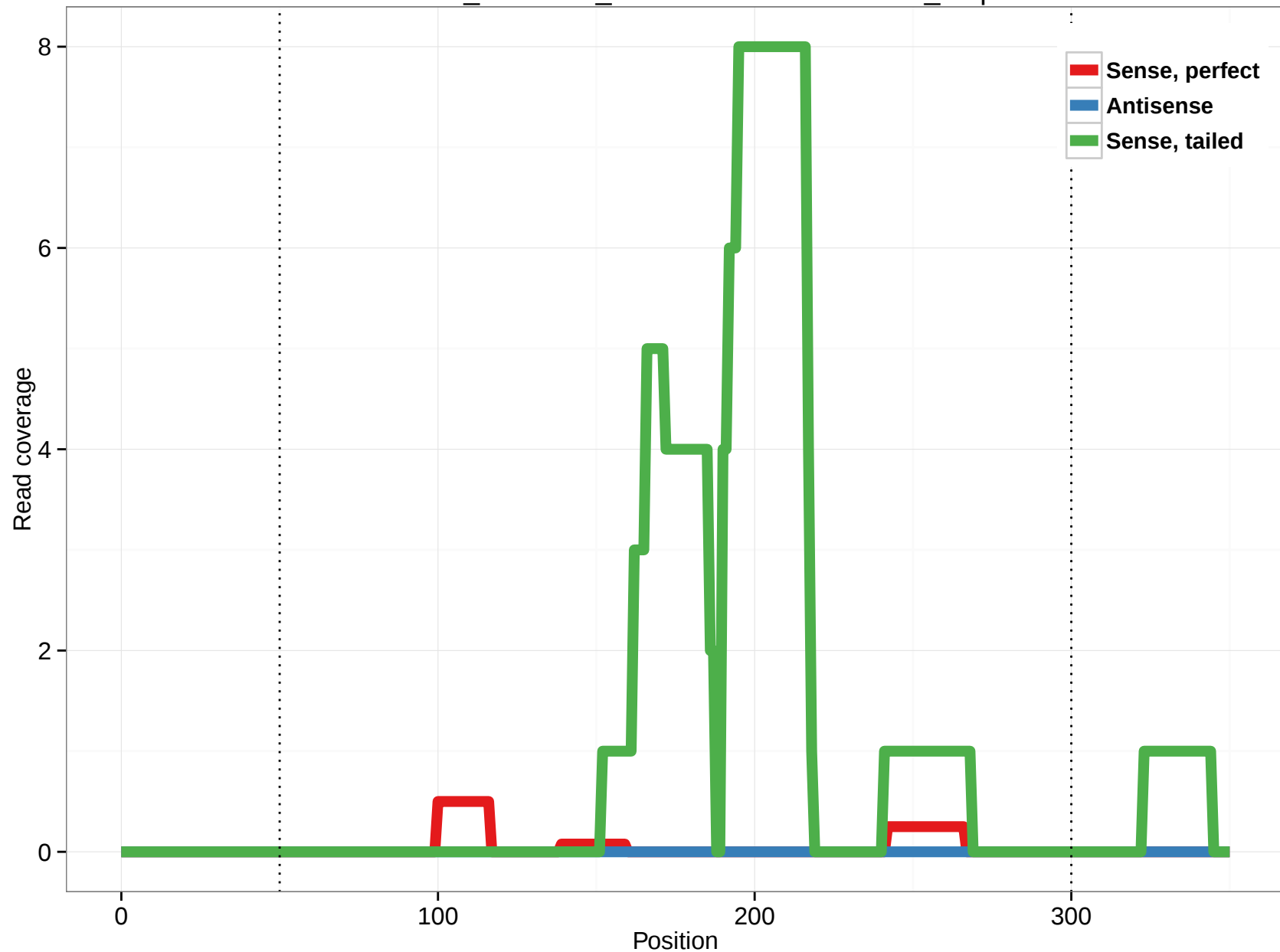
ornAna1_ensGene_ENSOANT00000011525_6.5p
