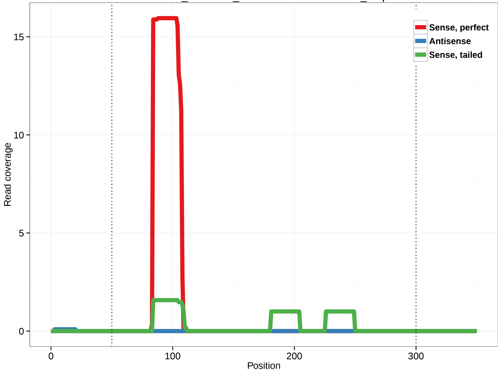
ornAna1_ensGene_ENSOANT00000011485_2.3p
