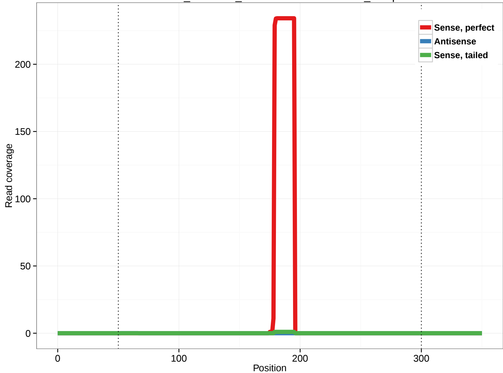
ornAna1_ensGene_ENSOANT00000011344_13.3p
