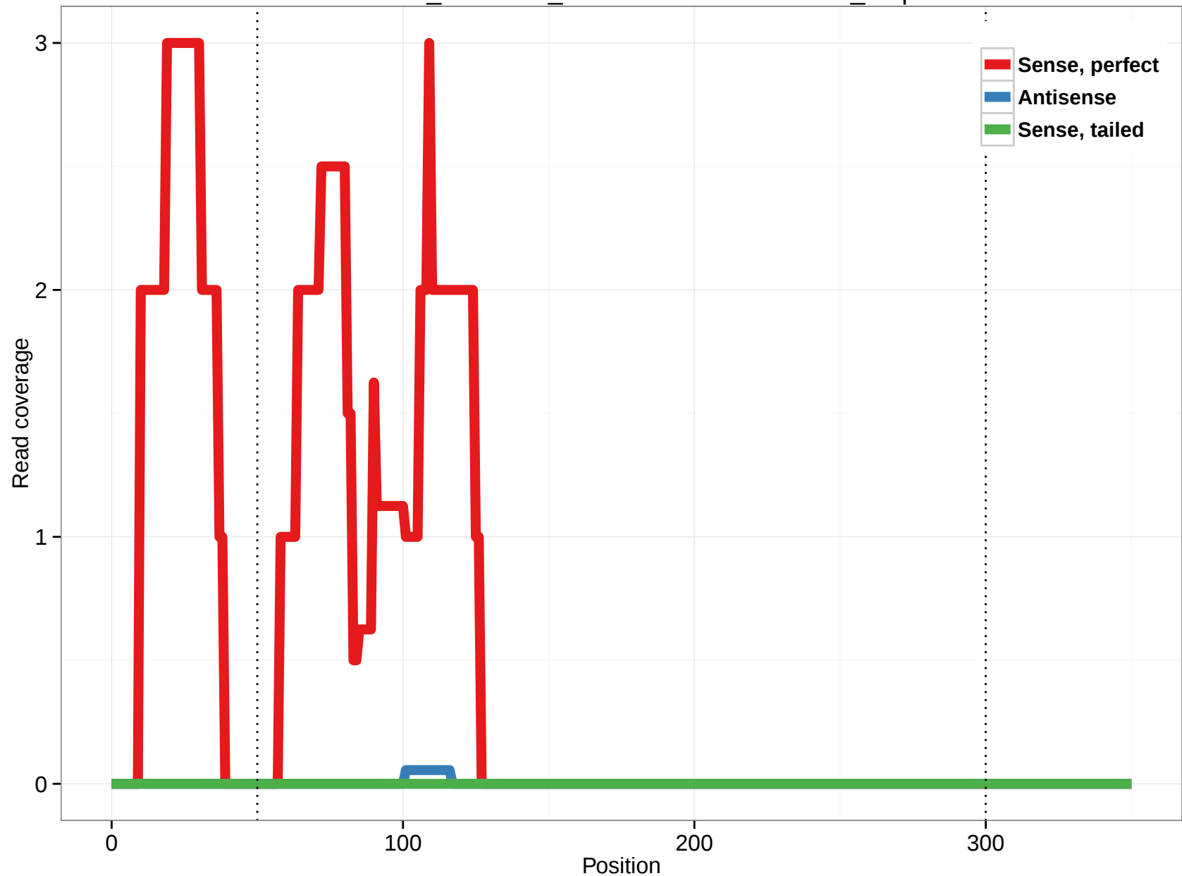
ornAna1_ensGene_ENSOANT00000011286_0.5p
