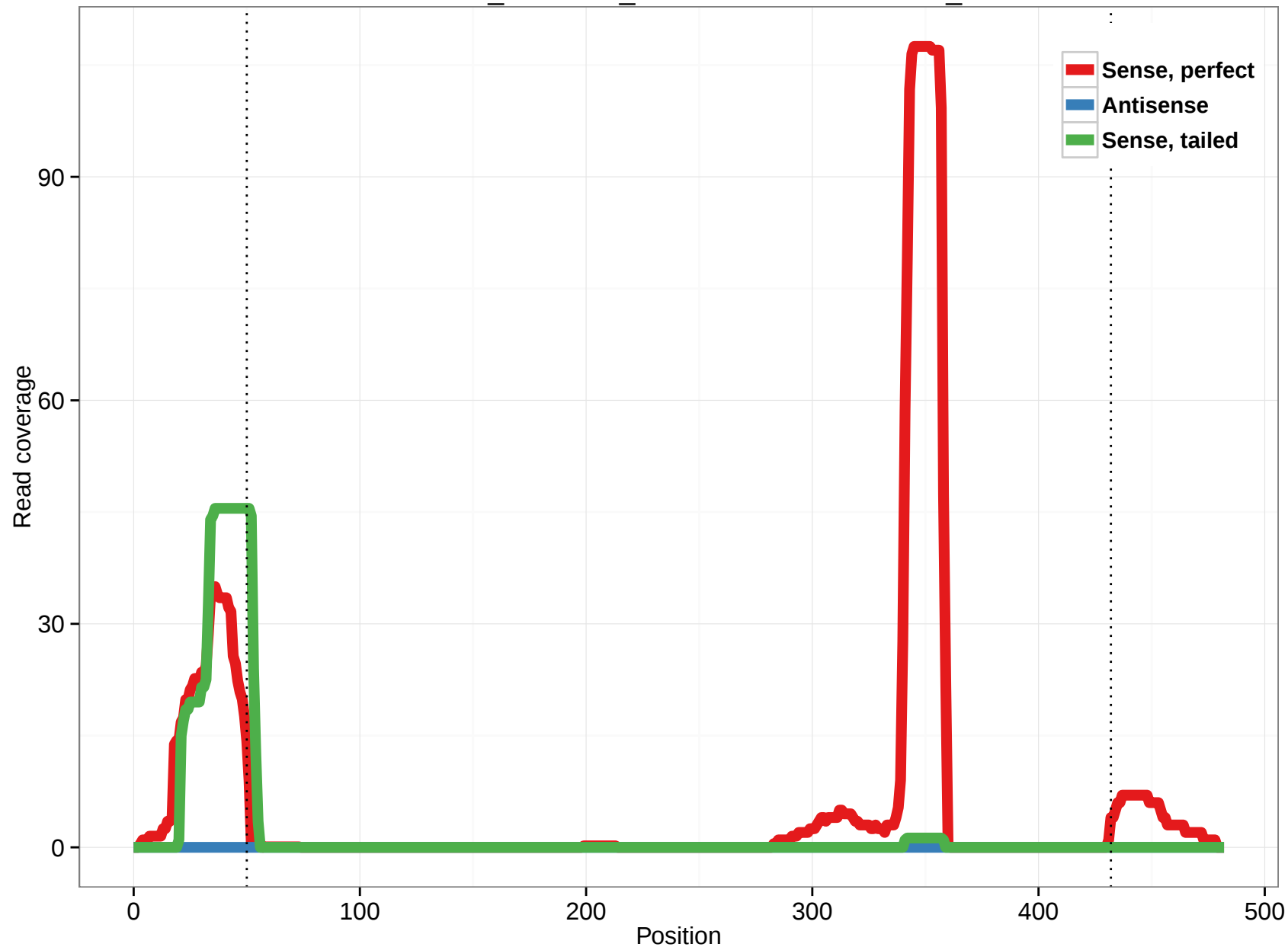
ornAna1_ensGene_ENSOANT00000011240_1
