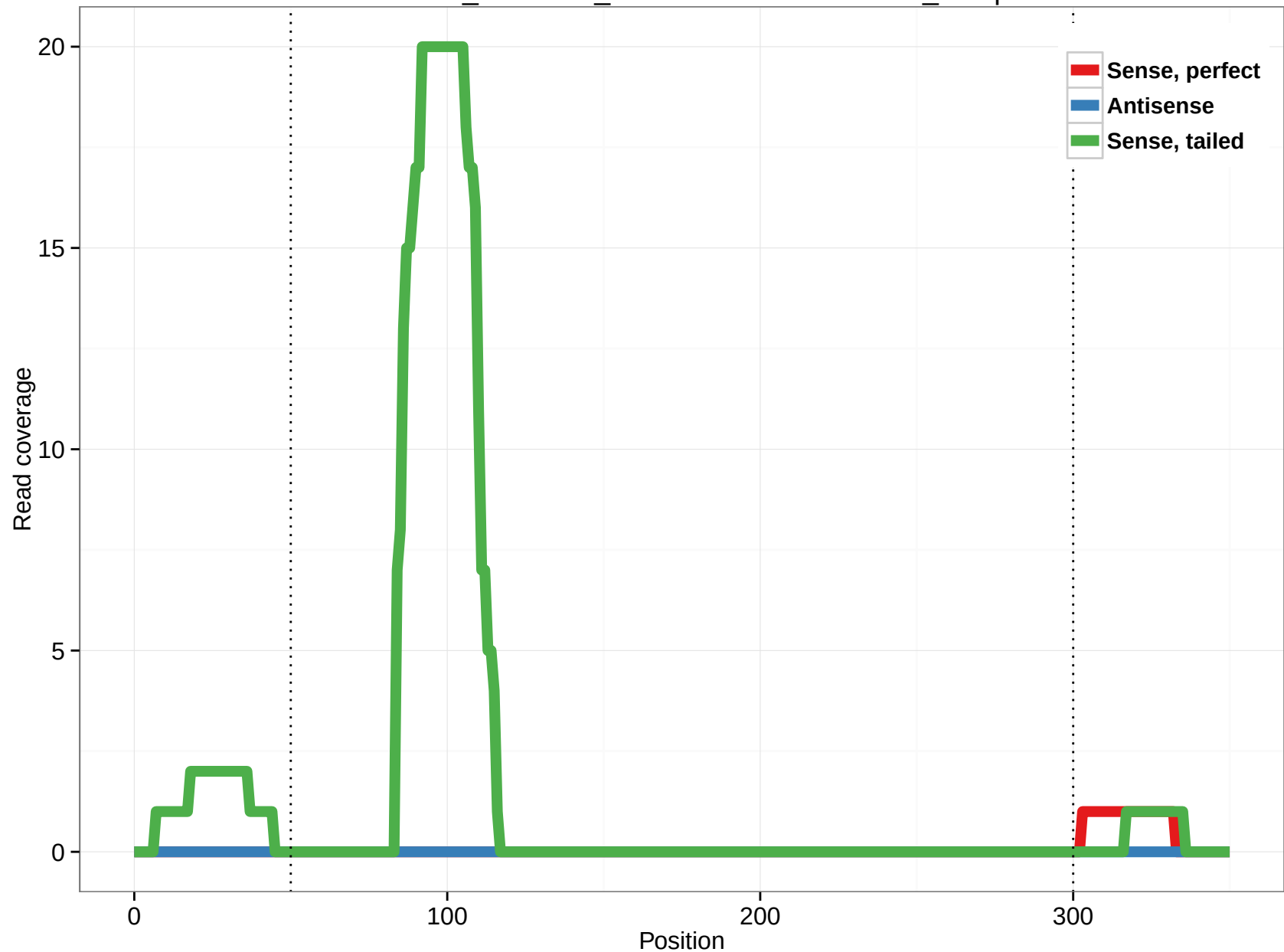
ornAna1_ensGene_ENSOANT00000011170_24.3p
