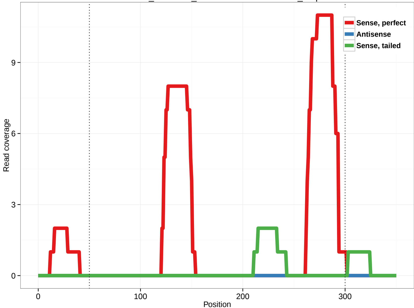
ornAna1_ensGene_ENSOANT00000011156_5.5p
