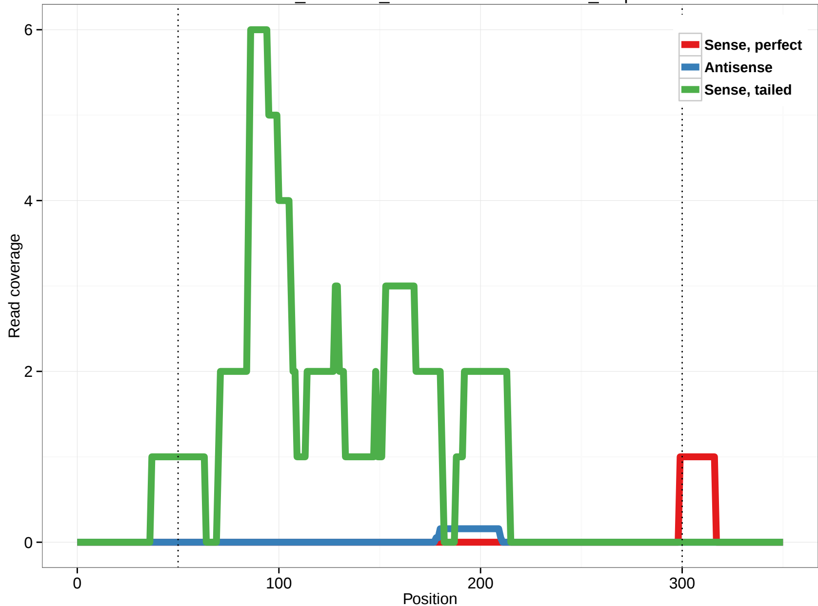
ornAna1_ensGene_ENSOANT00000011116_5.3p
