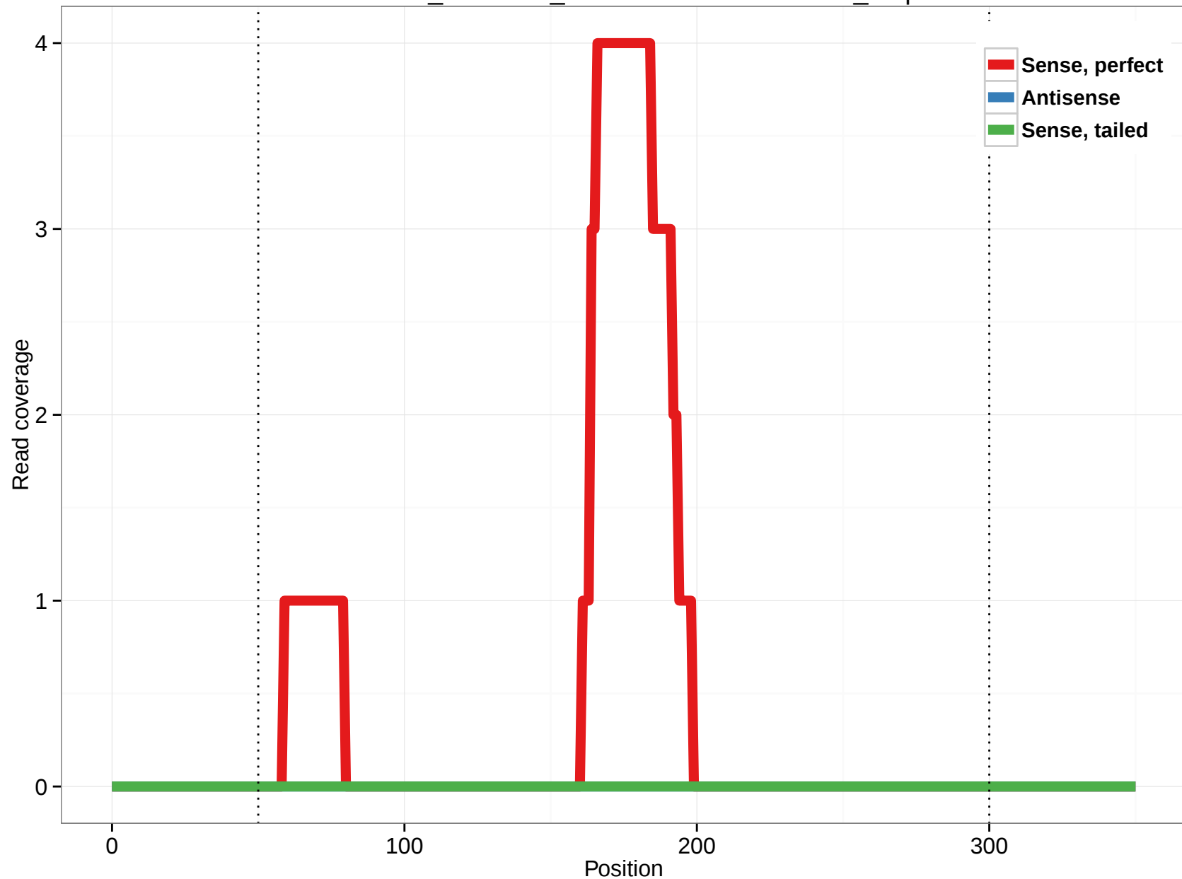
ornAna1_ensGene_ENSOANT00000011058_0.3p
