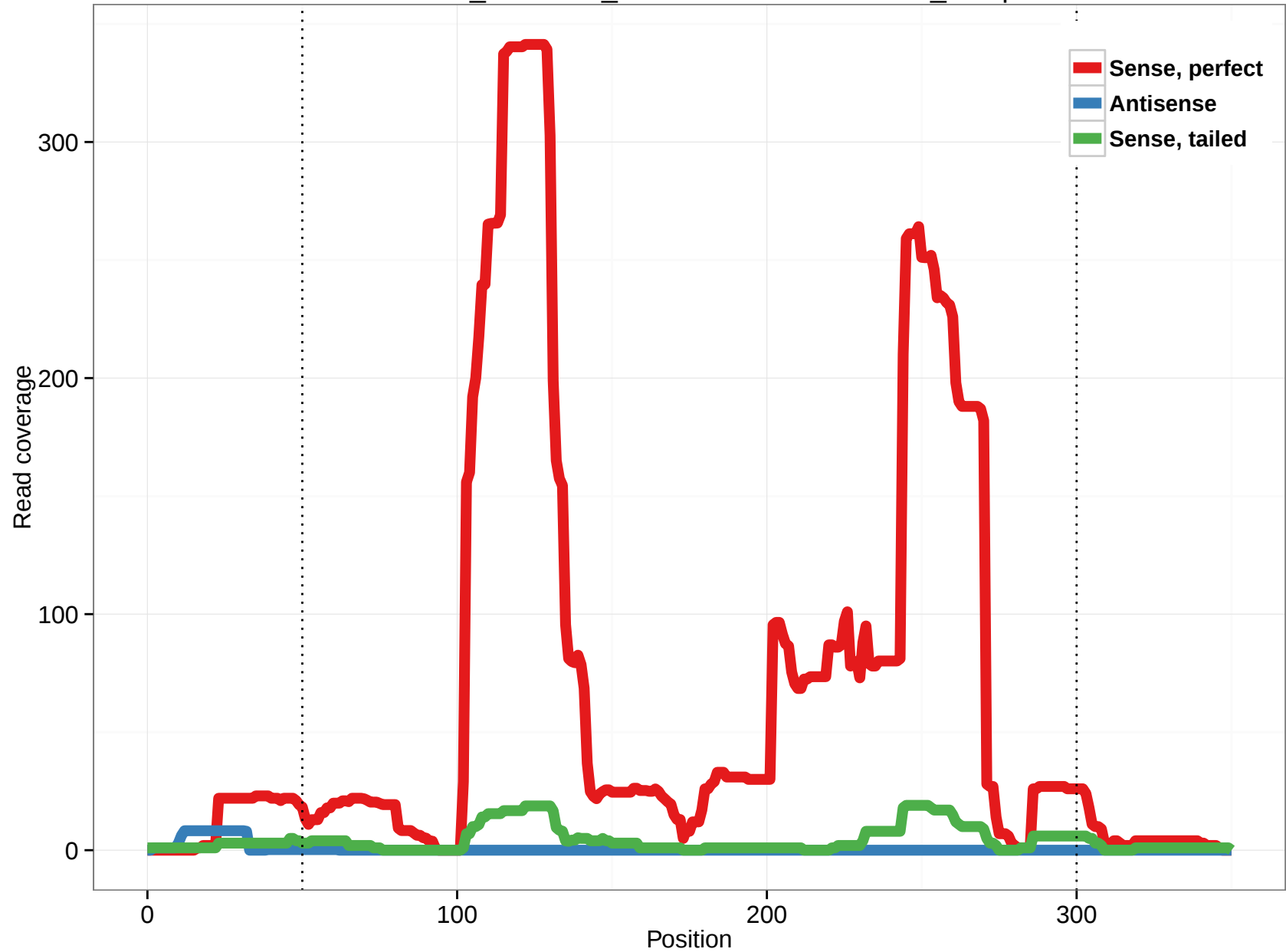
ornAna1_ensGene_ENSOANT00000011030_17.5p
