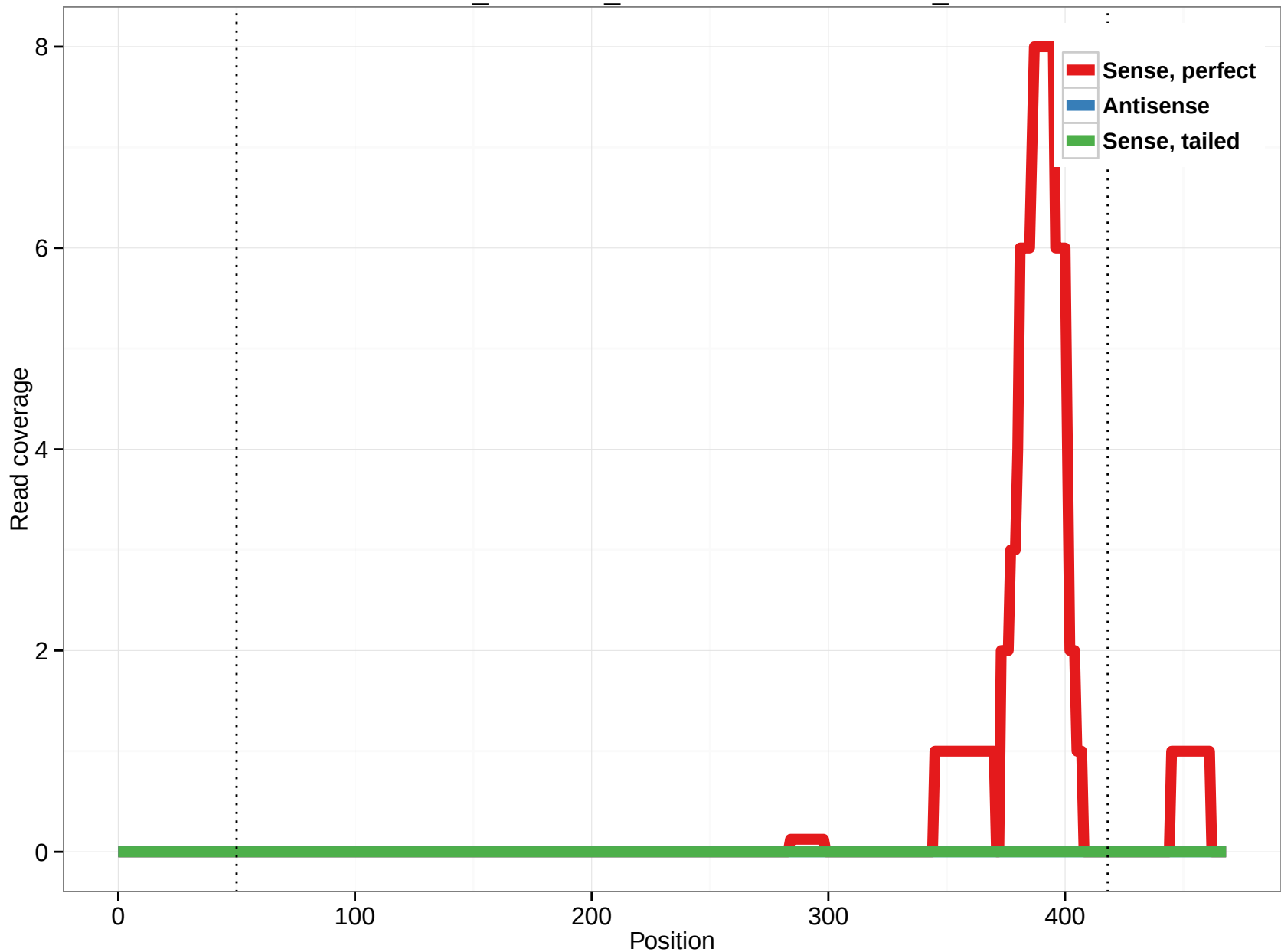
ornAna1_ensGene_ENSOANT00000011003_10
