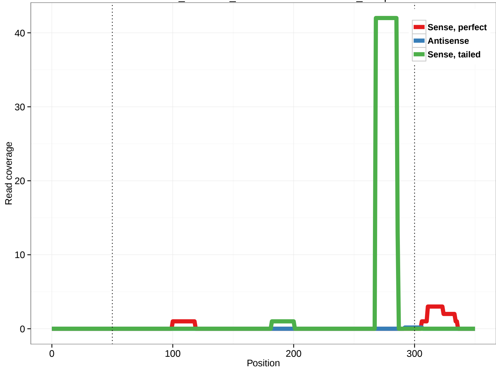
ornAna1_ensGene_ENSOANT00000010900_19.3p
