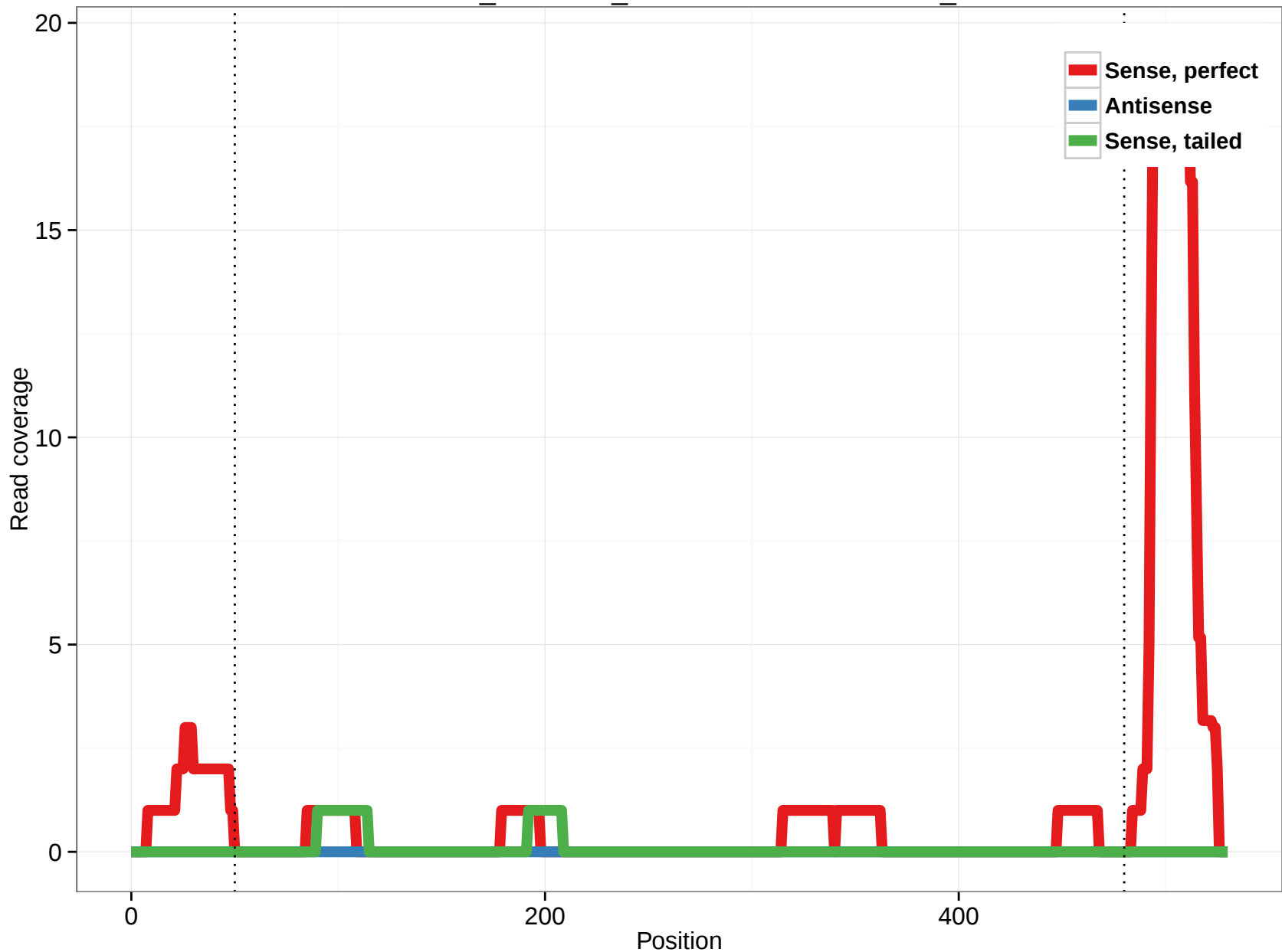
ornAna1_ensGene_ENSOANT00000010867_13
