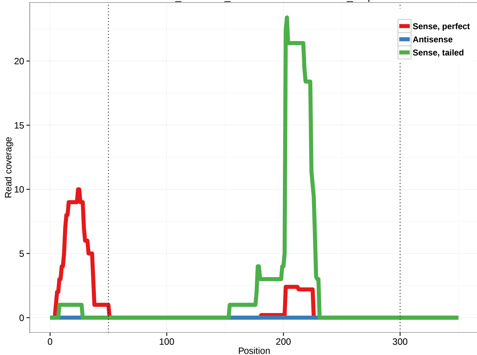
ornAna1_ensGene_ENSOANT00000010835_4.5p
