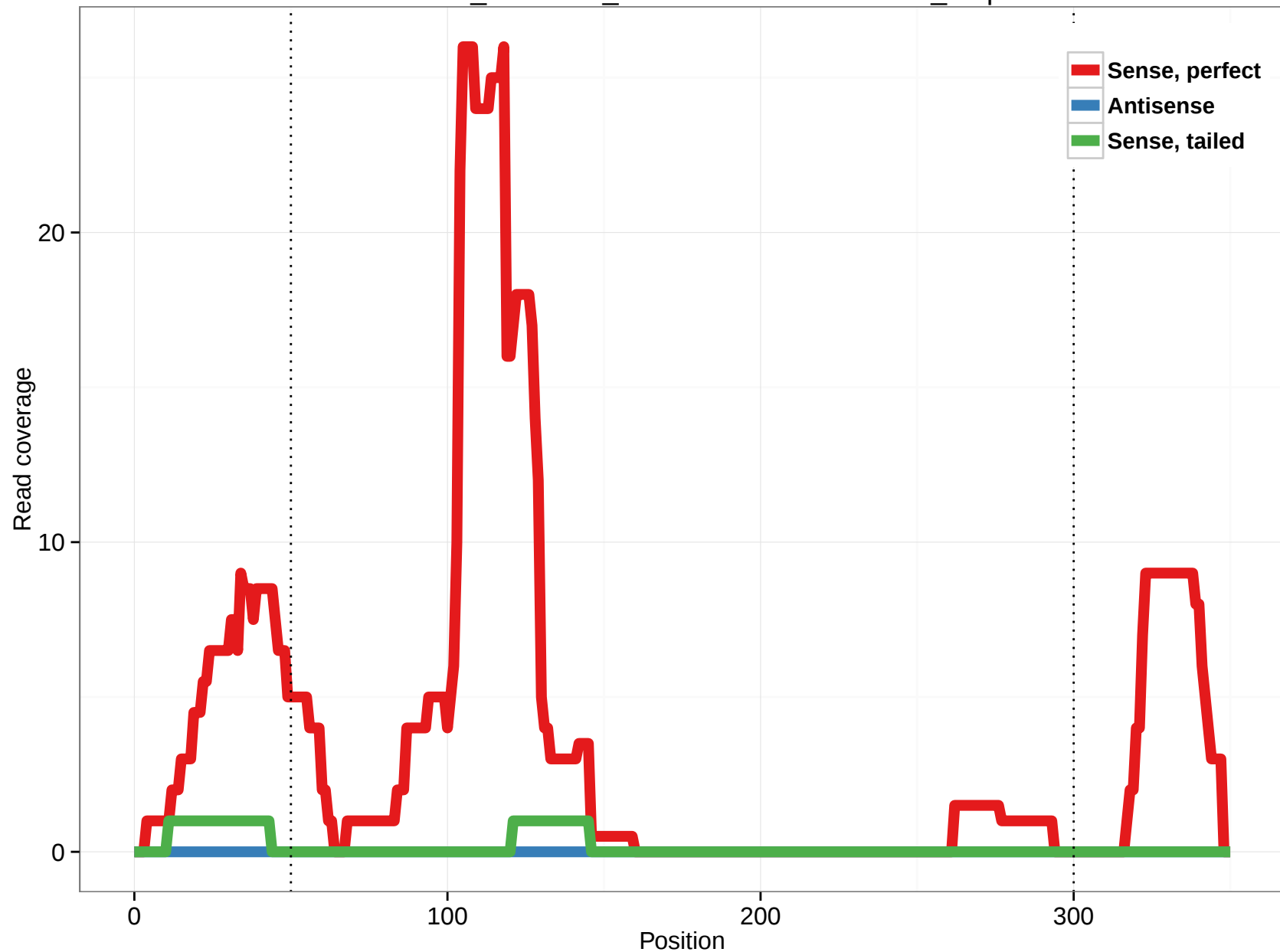
ornAna1_ensGene_ENSOANT00000010827_1.5p
