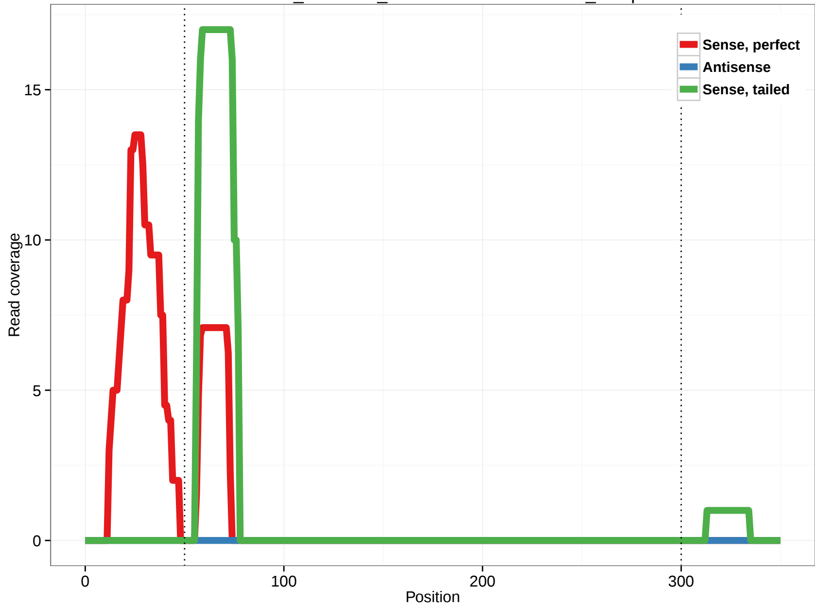
ornAna1_ensGene_ENSOANT00000010797_22.5p
