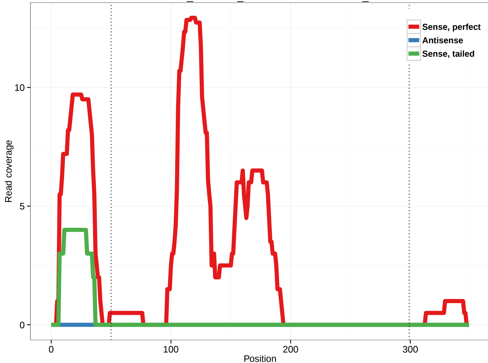
ornAna1_ensGene_ENSOANT00000010743_6
