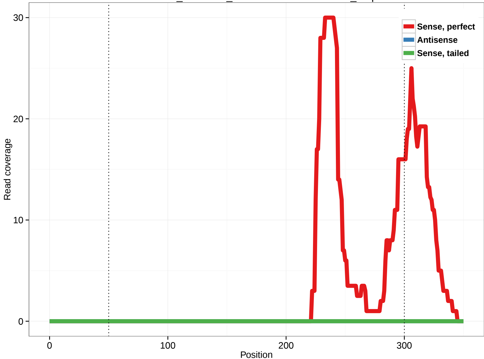
ornAna1_ensGene_ENSOANT00000010704_0.3p
