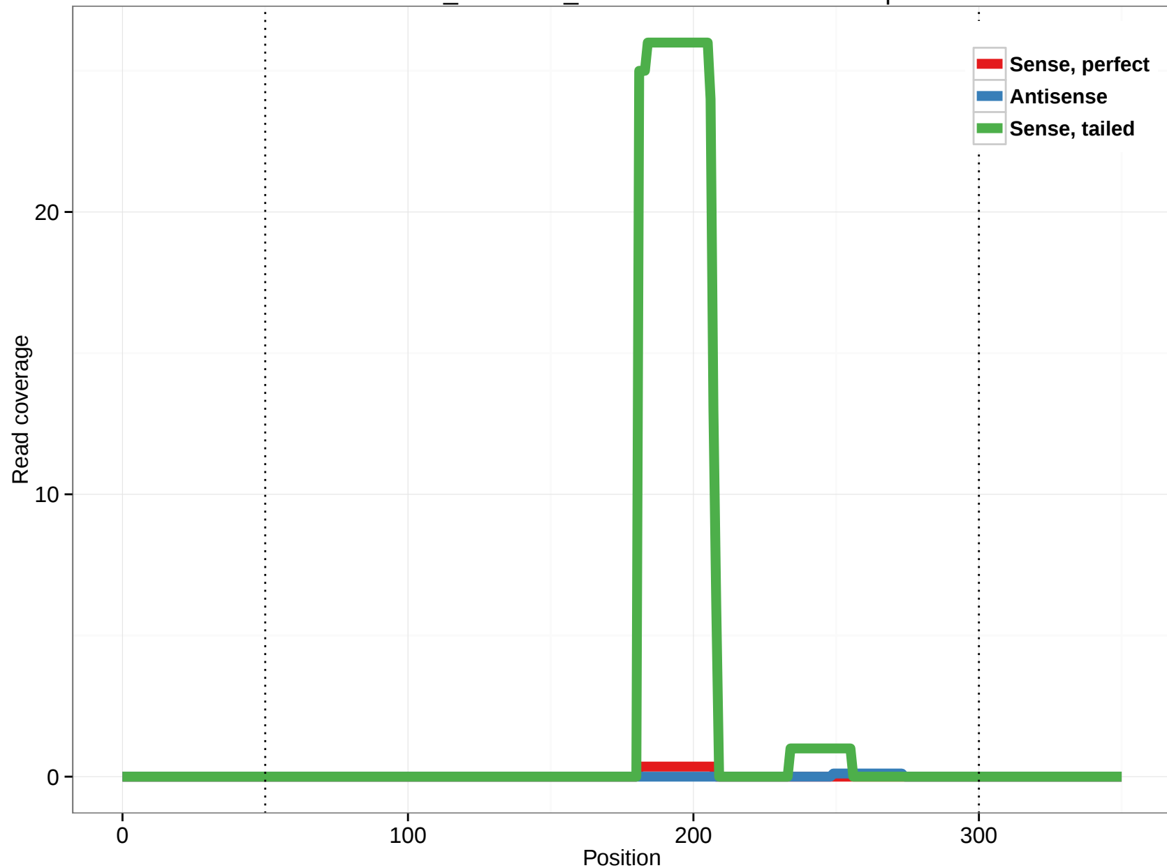
ornAna1_ensGene_ENSOANT00000010644.5p
