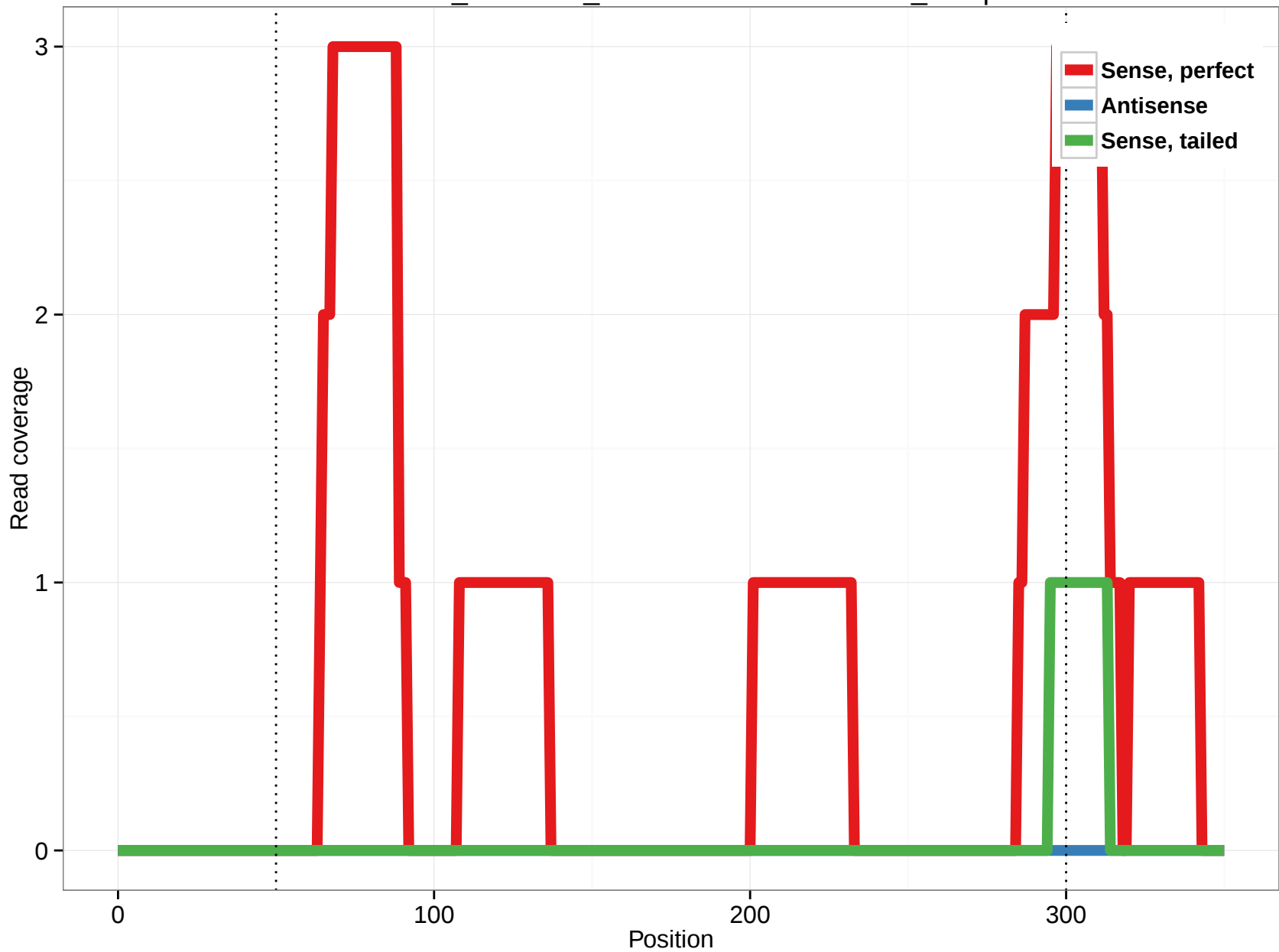
ornAna1_ensGene_ENSOANT00000010537_12.3p
