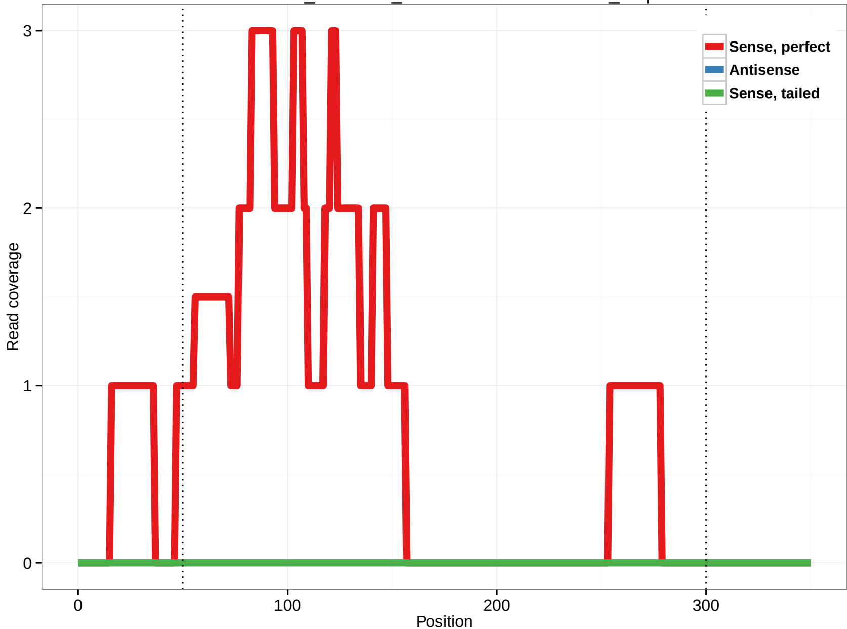
ornAna1_ensGene_ENSOANT00000010528_1.3p
