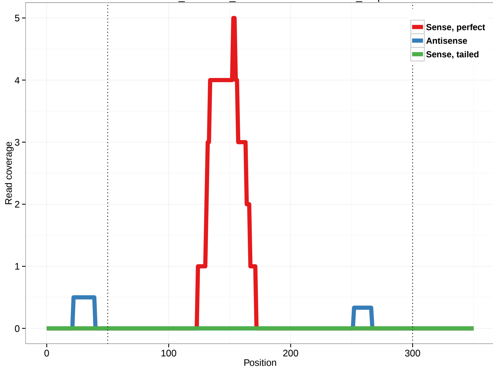
ornAna1_ensGene_ENSOANT00000010386_0.3p
