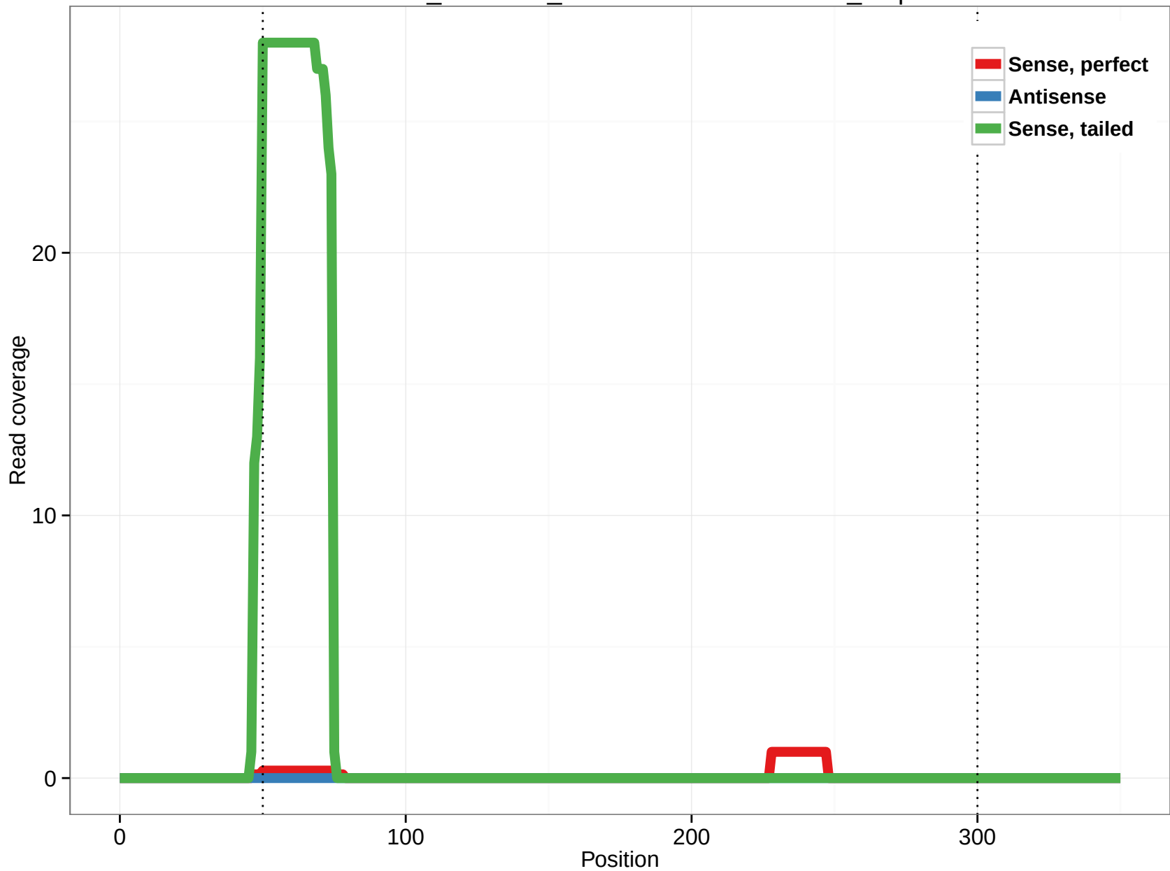
ornAna1_ensGene_ENSOANT00000010376_4.3p
