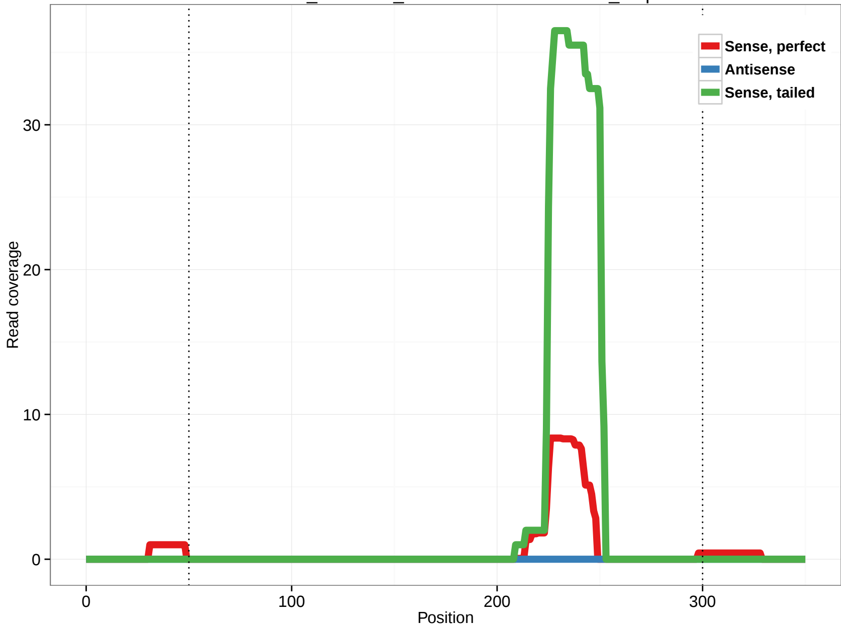
ornAna1_ensGene_ENSOANT00000010361_5.5p
