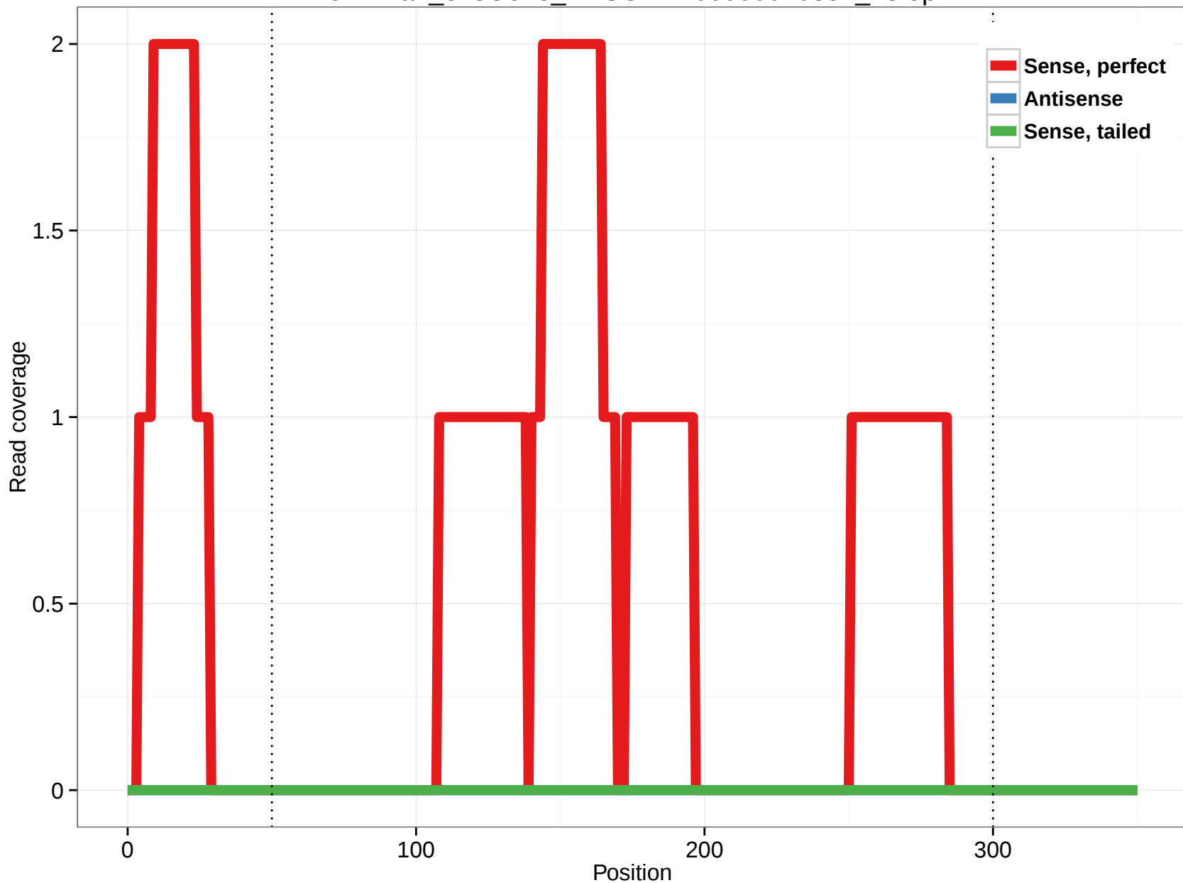
ornAna1_ensGene_ENSOANT00000010352_13.5p
