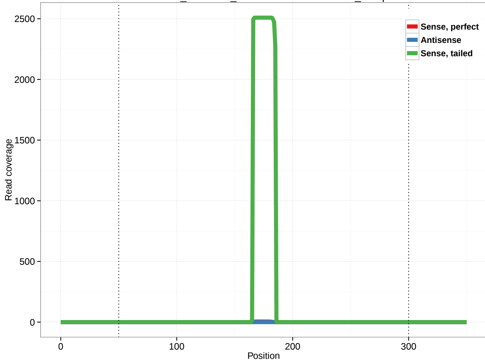
ornAna1_ensGene_ENSOANT00000010344_12.5p
