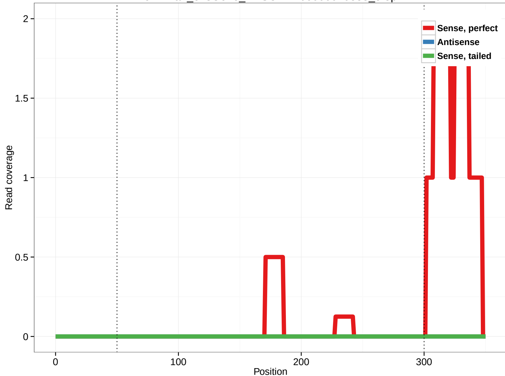
ornAna1_ensGene_ENSOANT00000010338_5.3p
