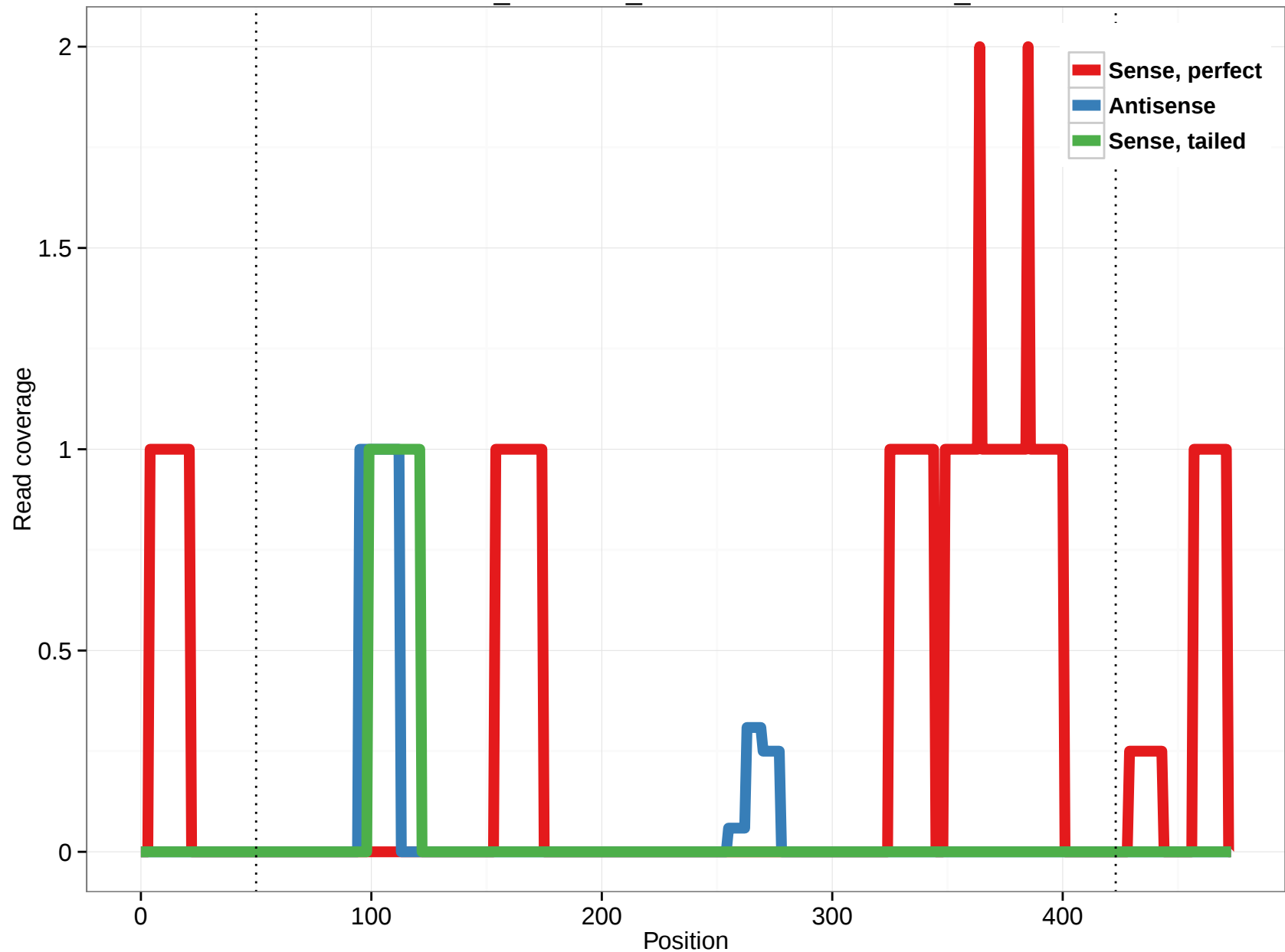
ornAna1_ensGene_ENSOANT00000010336_0
