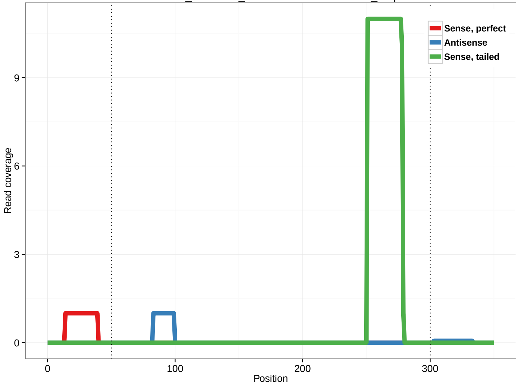
ornAna1_ensGene_ENSOANT00000010289_8.5p
