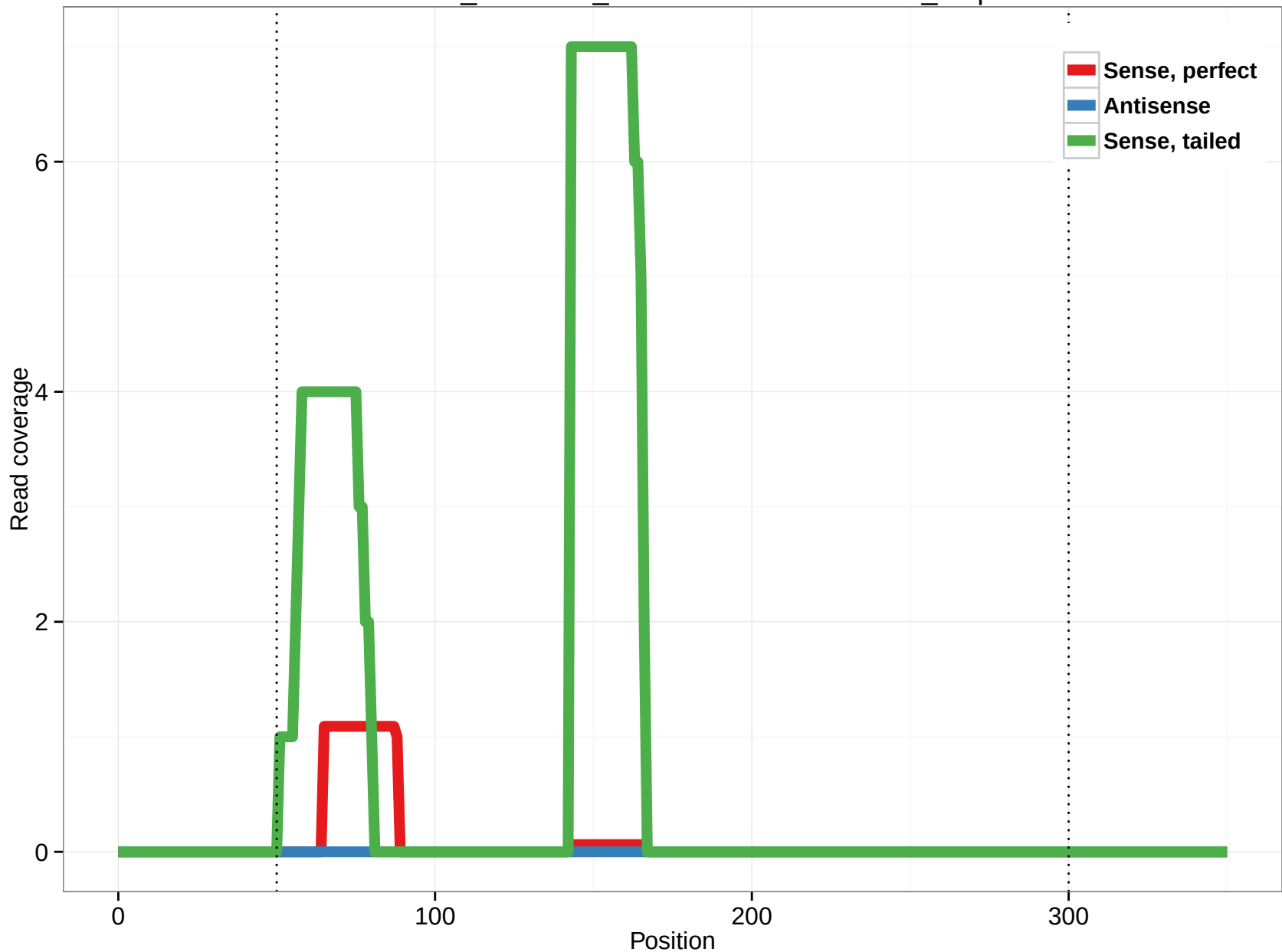
ornAna1_ensGene_ENSOANT00000010288_9.3p
