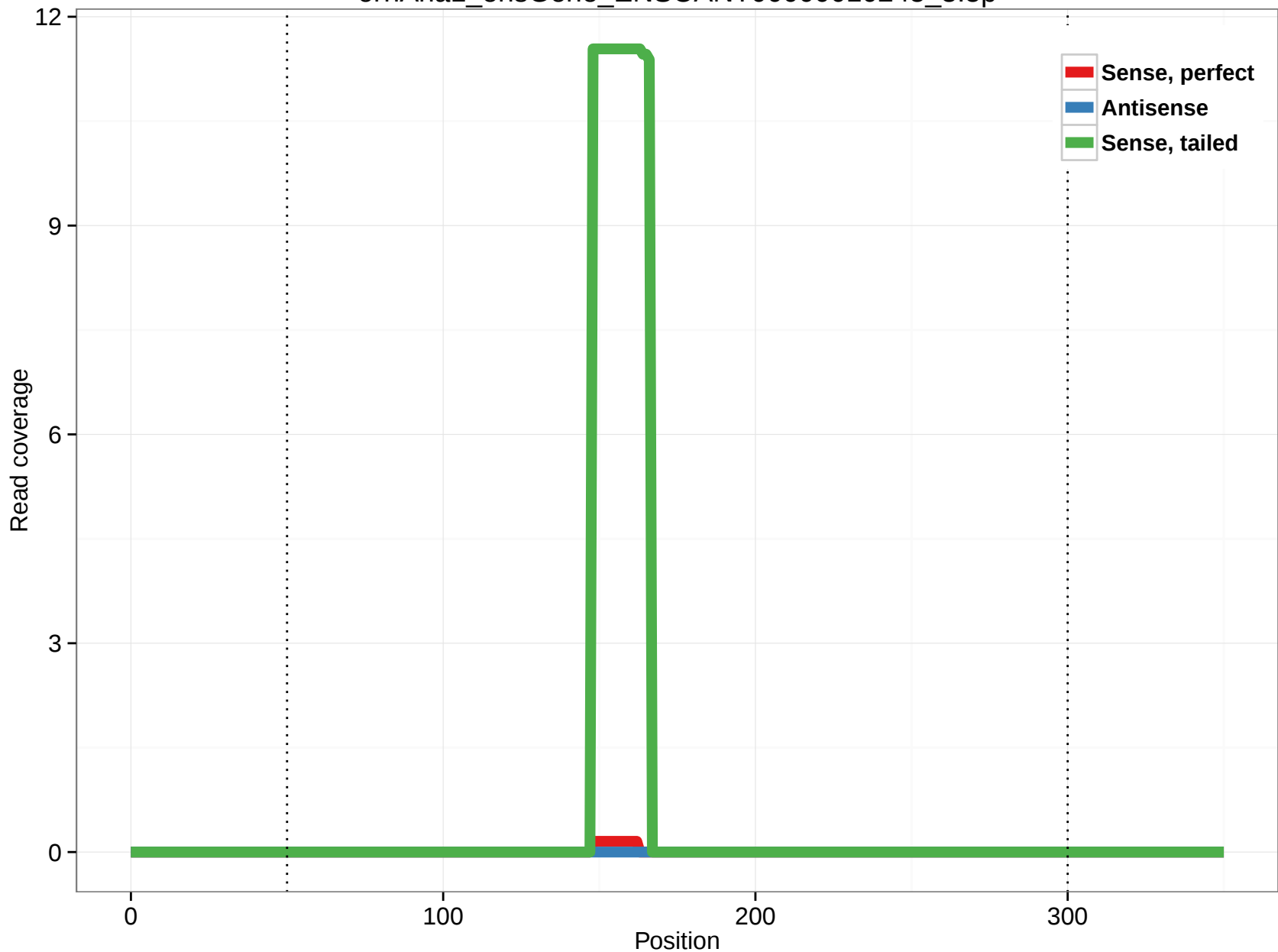
ornAna1_ensGene_ENSOANT00000010245_3.5p
