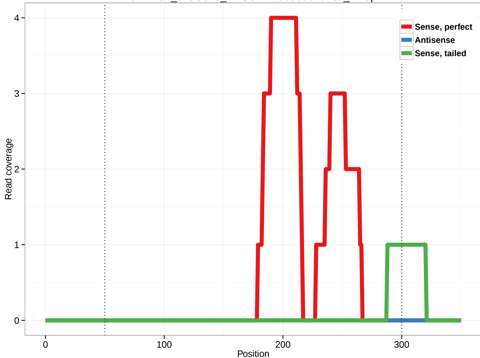
ornAna1_ensGene_ENSOANT00000010232_14.3p
