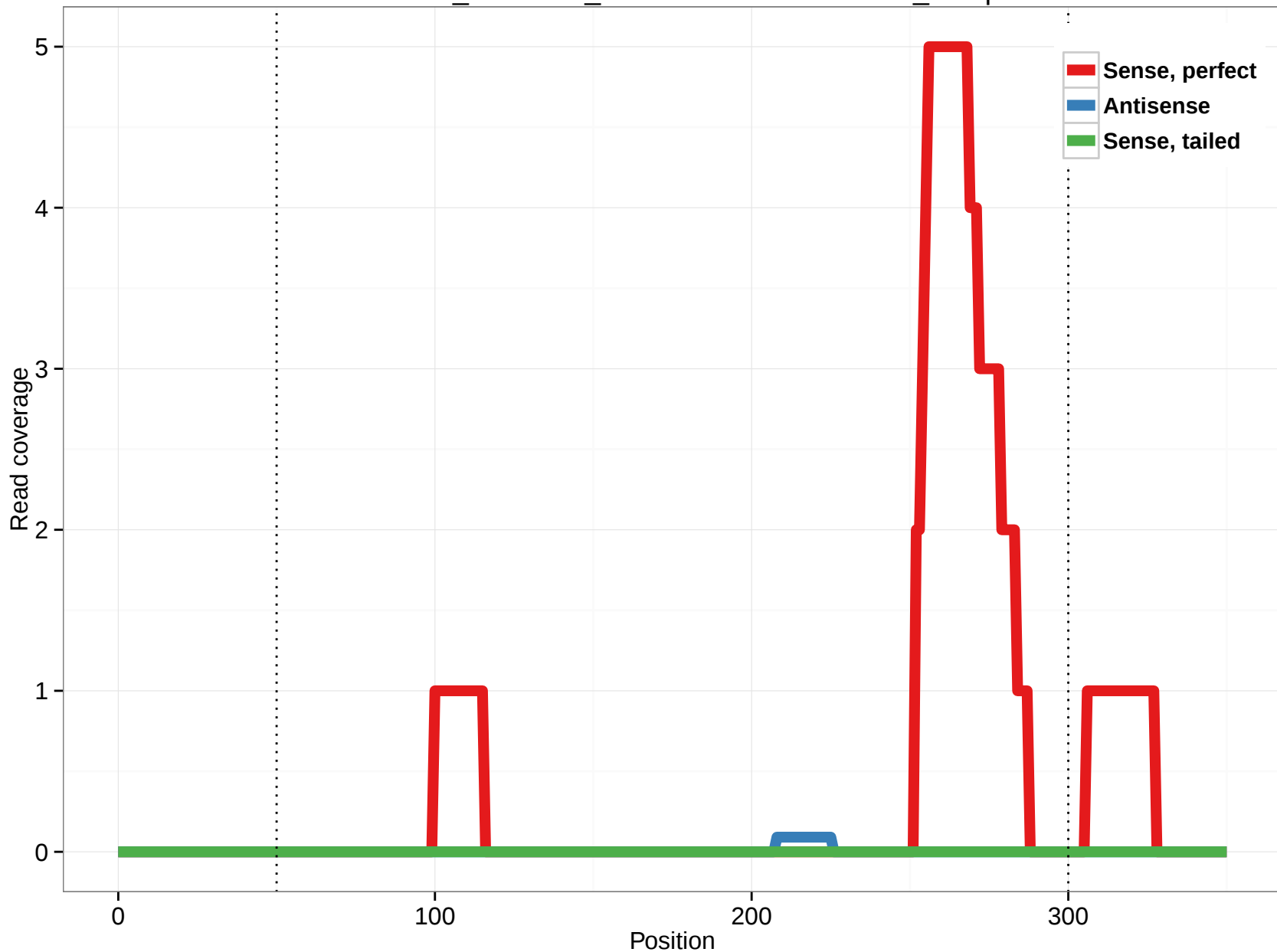
ornAna1_ensGene_ENSOANT00000010192_14.3p
