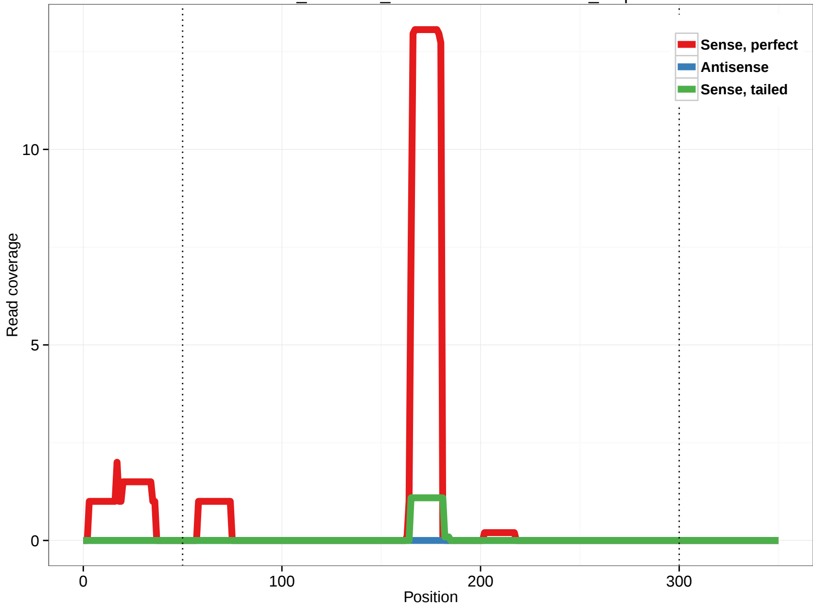
ornAna1_ensGene_ENSOANT00000010192_1.3p
