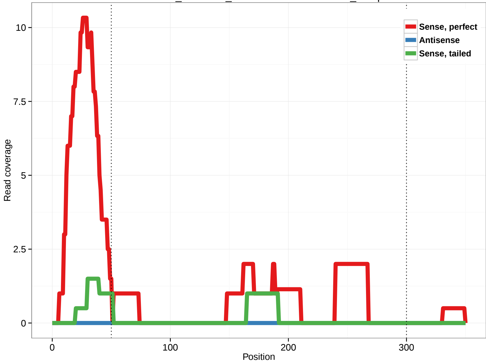
ornAna1_ensGene_ENSOANT00000010136_13.5p
