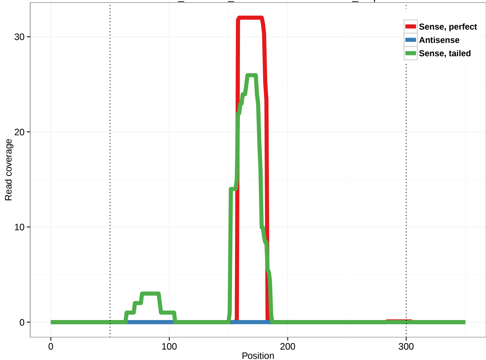
ornAna1_ensGene_ENSOANT00000009963_1.5p
