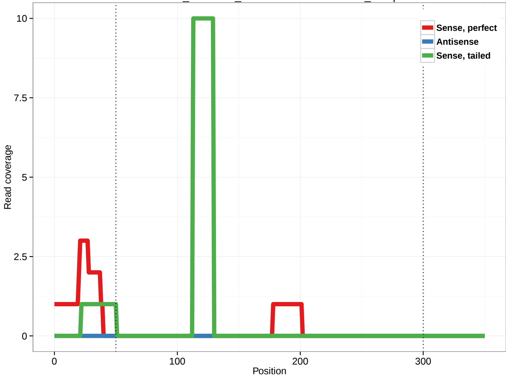
ornAna1_ensGene_ENSOANT00000009954_20.5p
