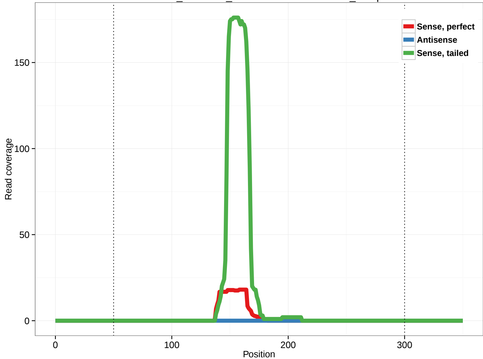
ornAna1_ensGene_ENSOANT00000009921_11.3p
