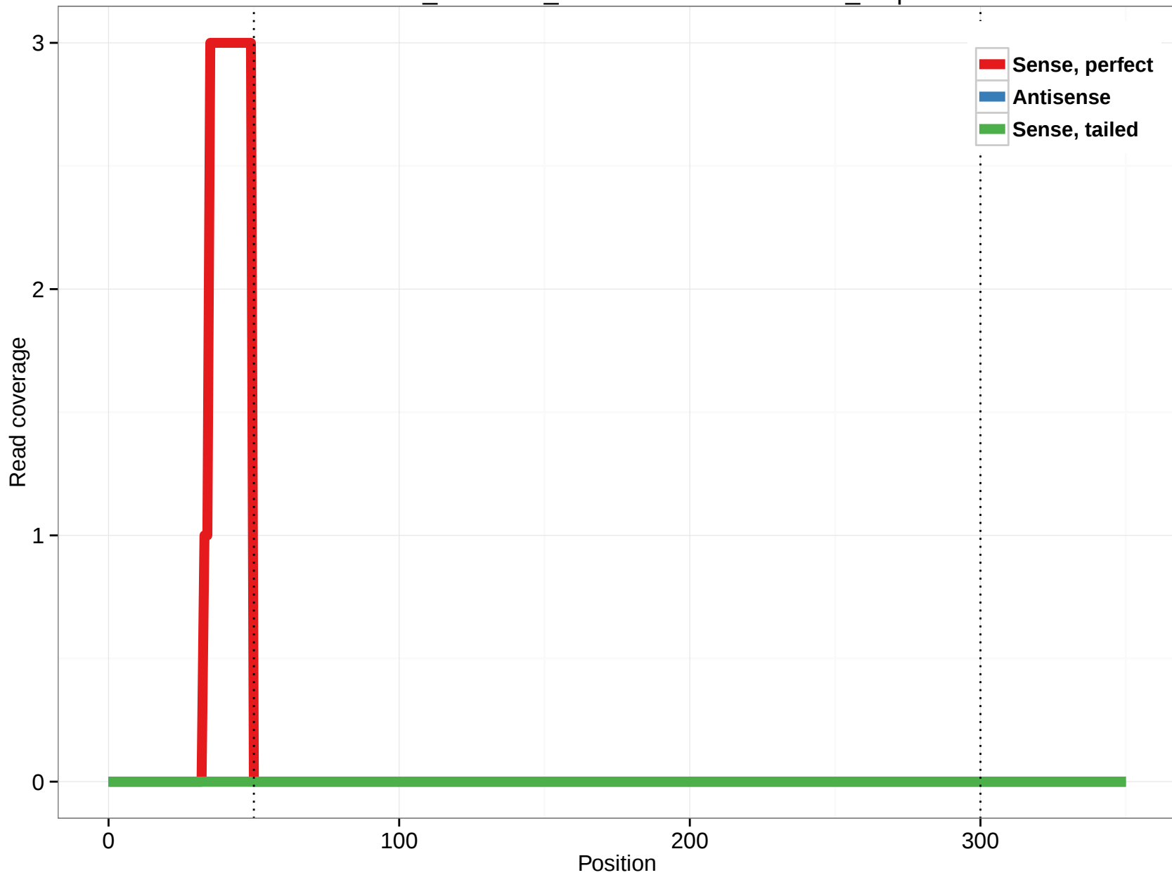
ornAna1_ensGene_ENSOANT00000009893_4.5p
