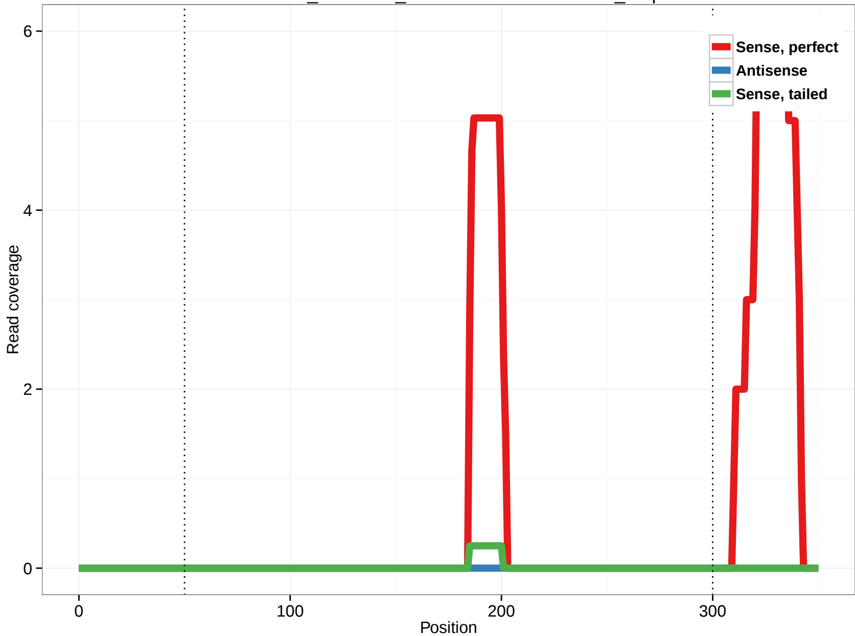
ornAna1_ensGene_ENSOANT00000009851_0.3p
