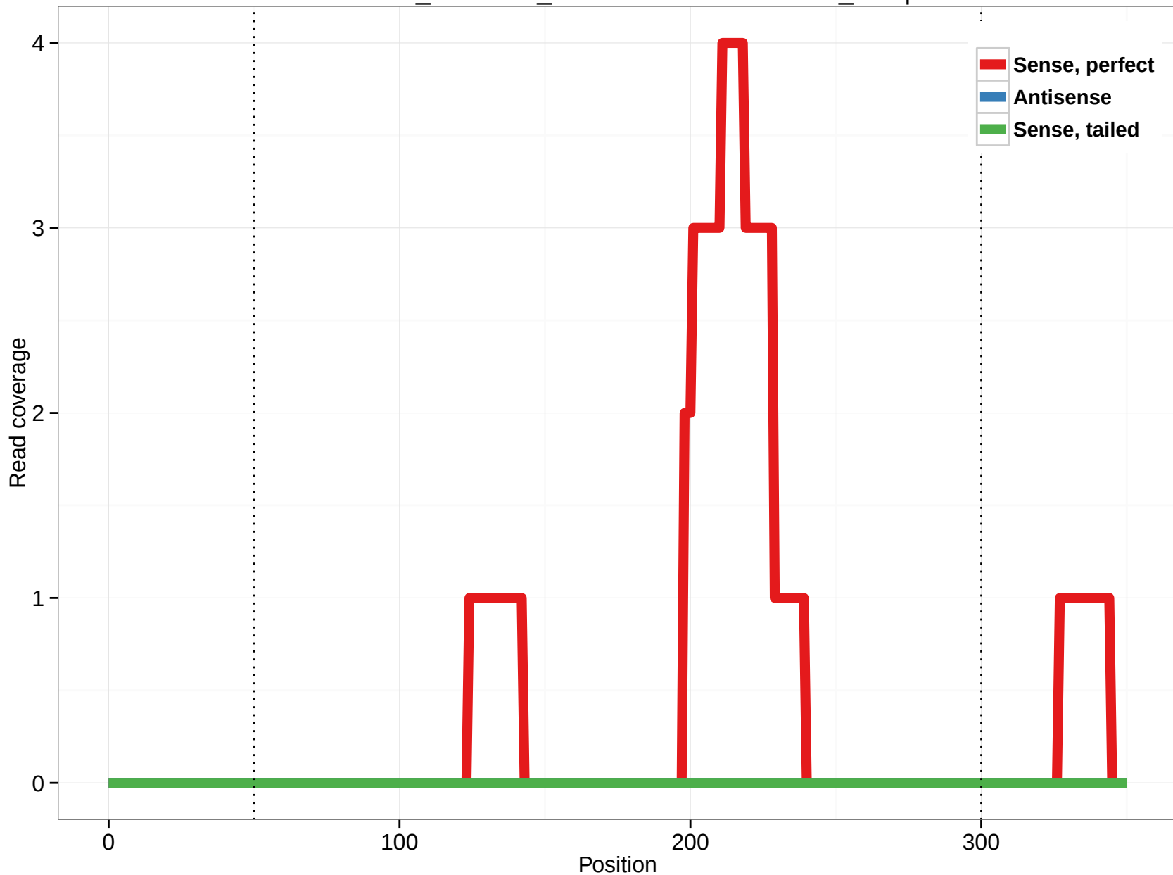
ornAna1_ensGene_ENSOANT00000009831_15.3p
