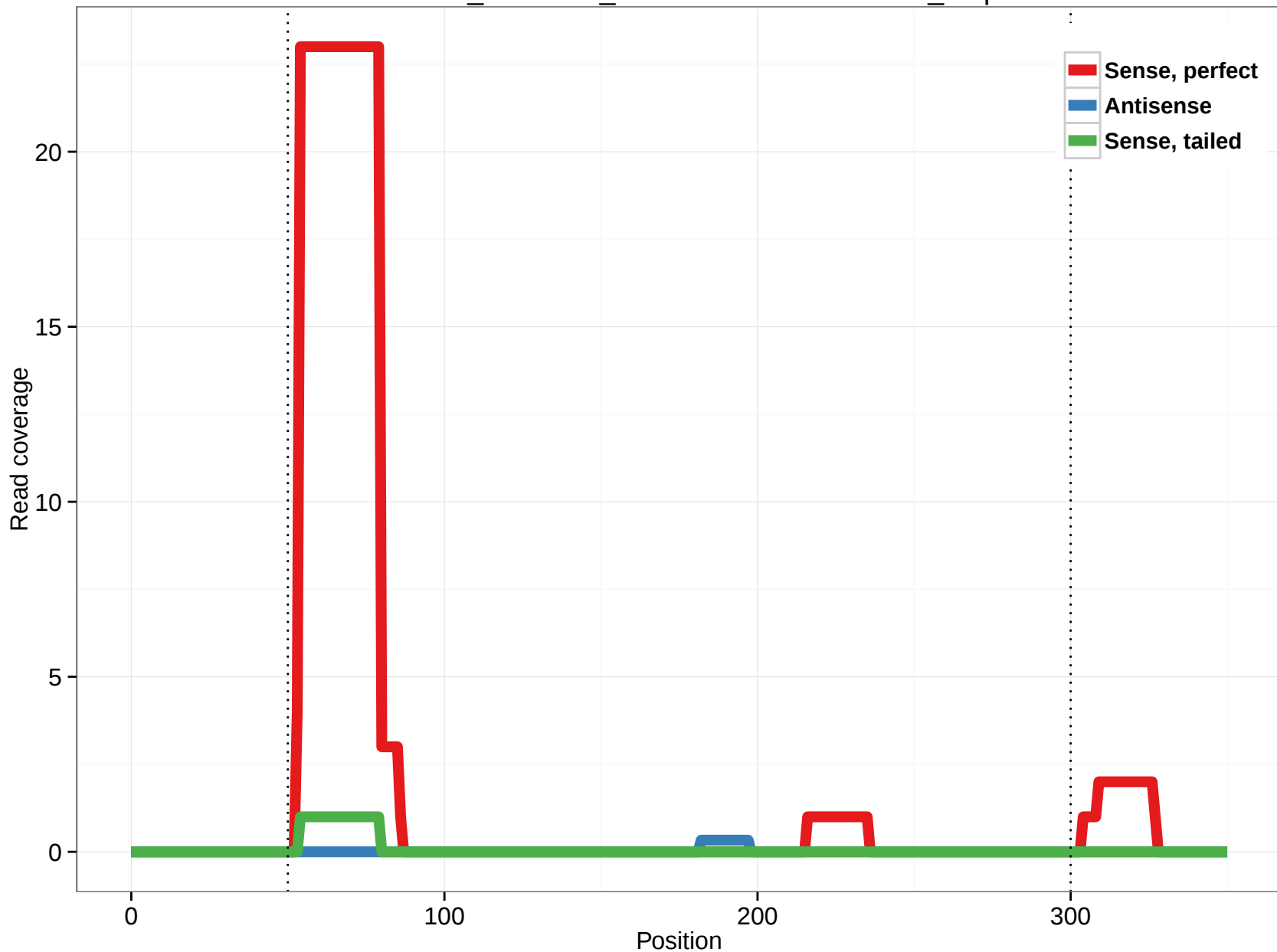
ornAna1_ensGene_ENSOANT00000009738_3.3p
