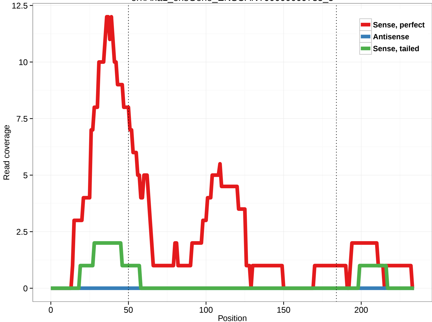
ornAna1_ensGene_ENSOANT00000009733_5
