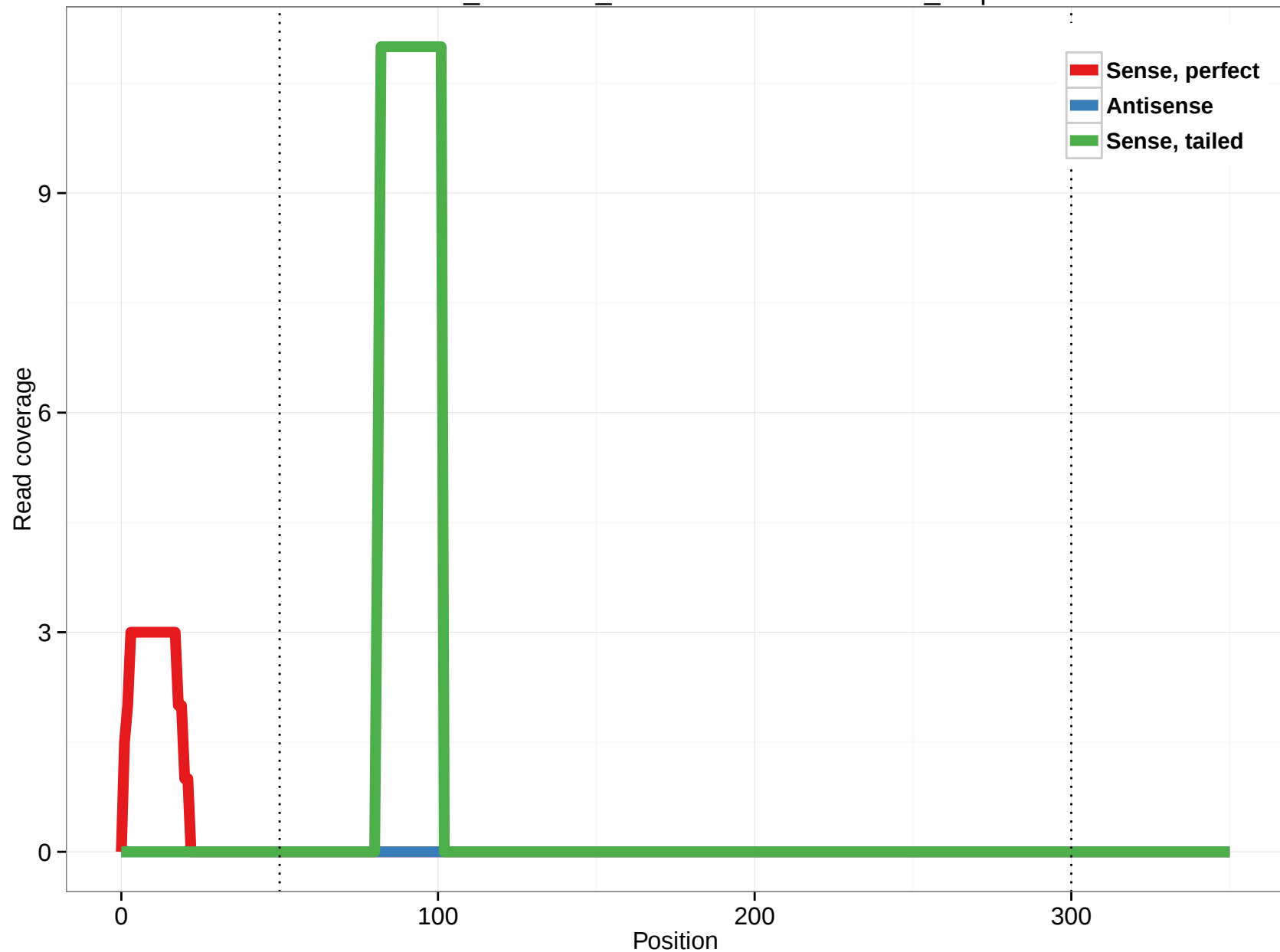
ornAna1_ensGene_ENSOANT00000009709_0.5p
